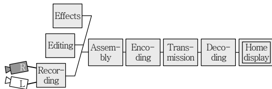
(그림 1) 3DTV broadcasting chain[2]
